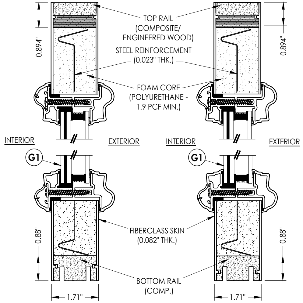
4 VERTICAL CROSS SECTION
